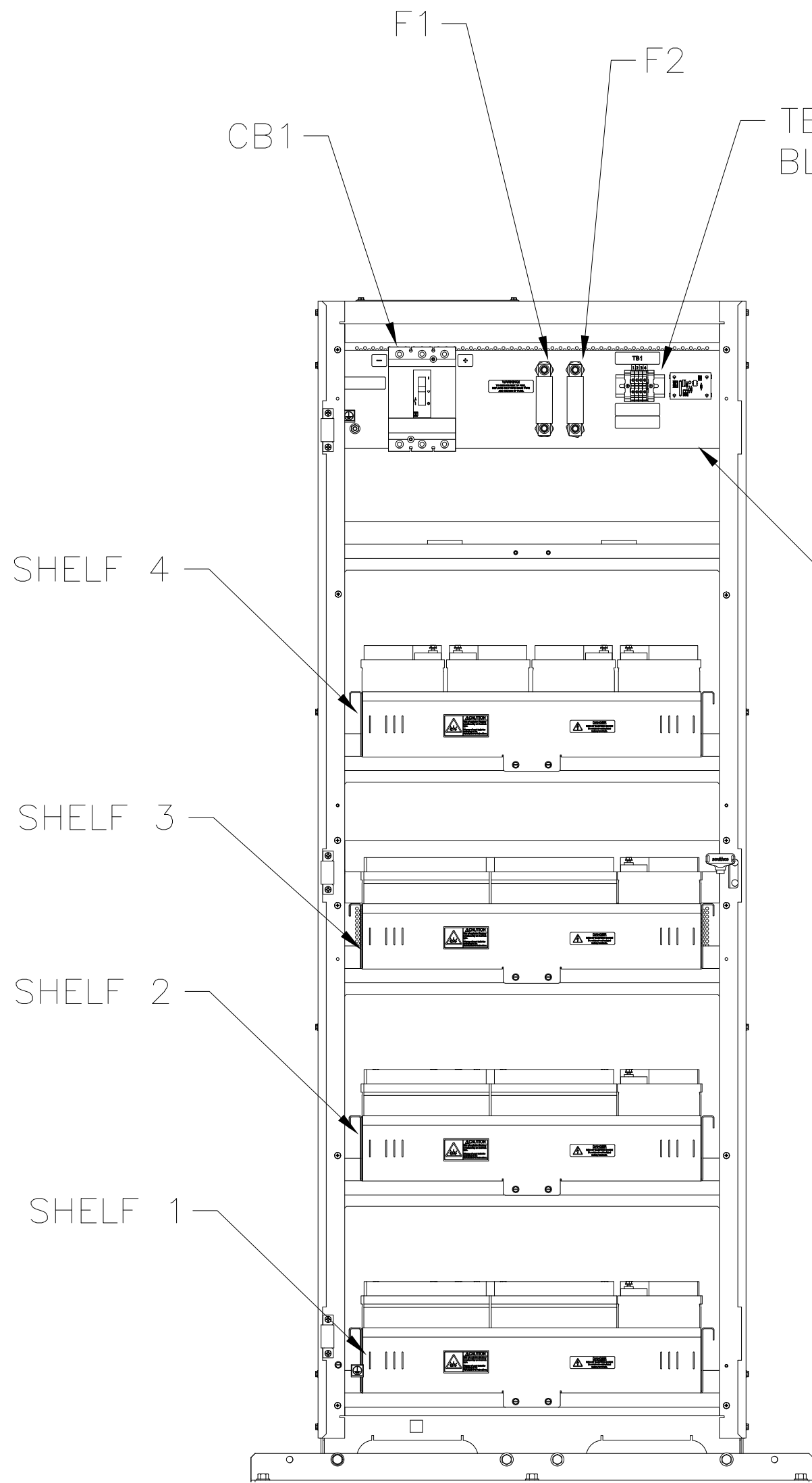
FRONT VIEW COVERS REMOVED
